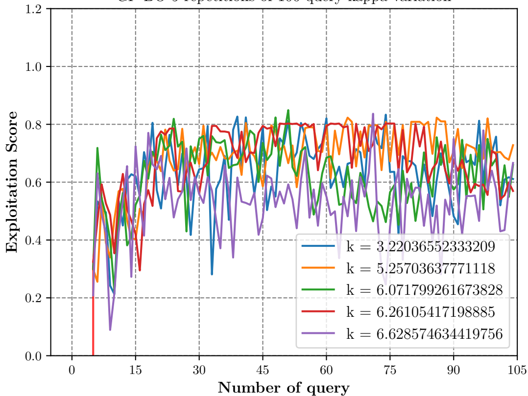
GP-BO 5 repetitions of 100 query kappa variation
